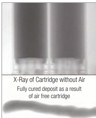
X-Ray of Cartridge with Air Trapped air creates a lower quality deposit
